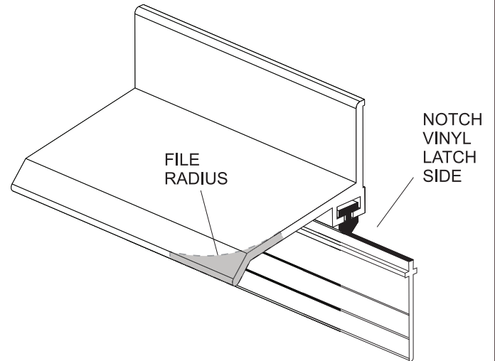
Figure #4 - FSD Vinyl Notching
