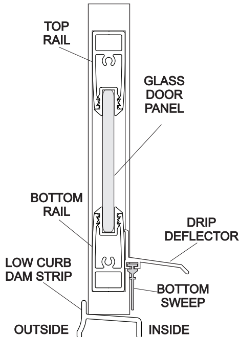
Figure #3 - FSD Side View
