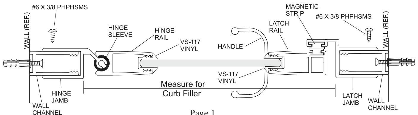
Figure #2 - FSD Shower Door Assembly - Top View
