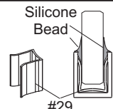
Silicone Bead #29 Wet Glazing parts detail Page 7
