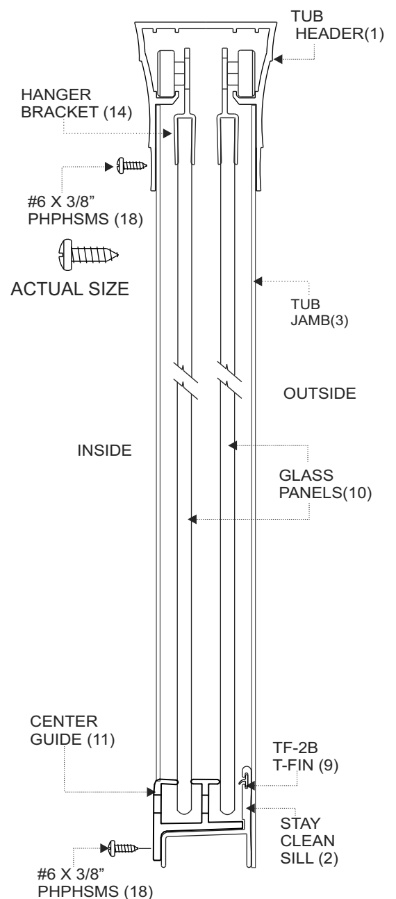
ELEVATION VIEW
