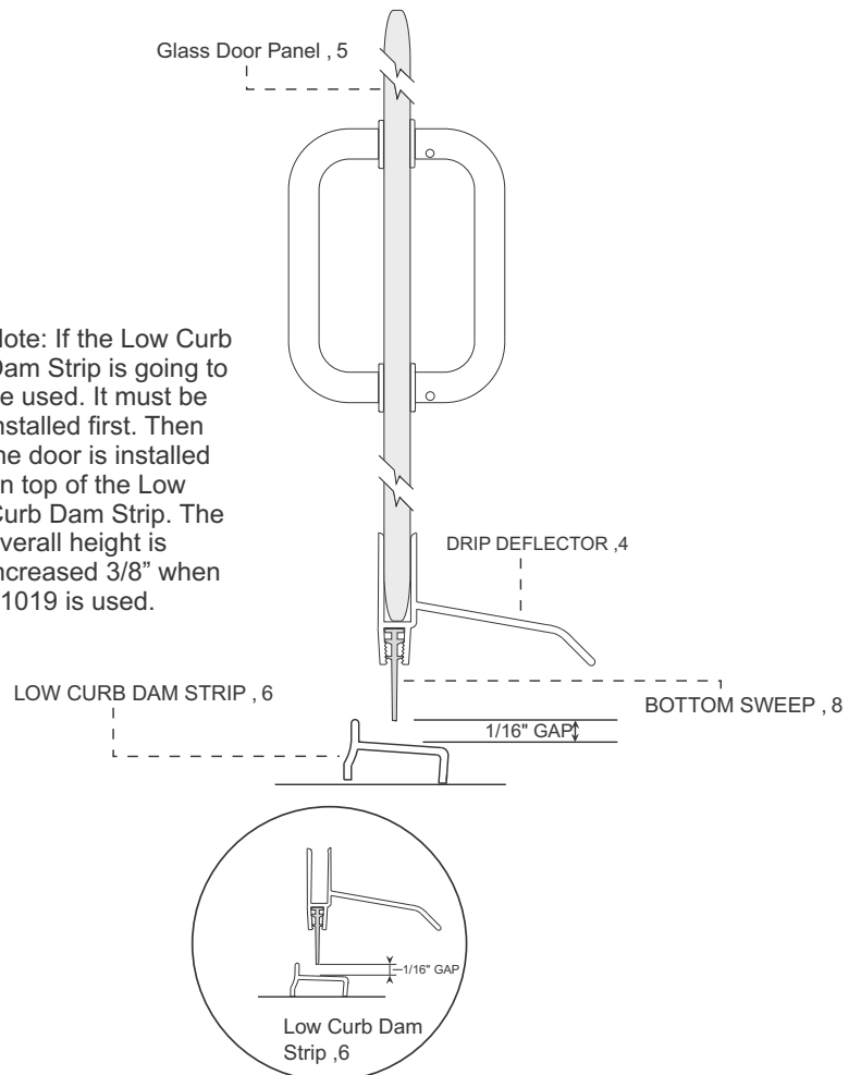
Fig. #5 - Bottom Sweep Gap Clearance
