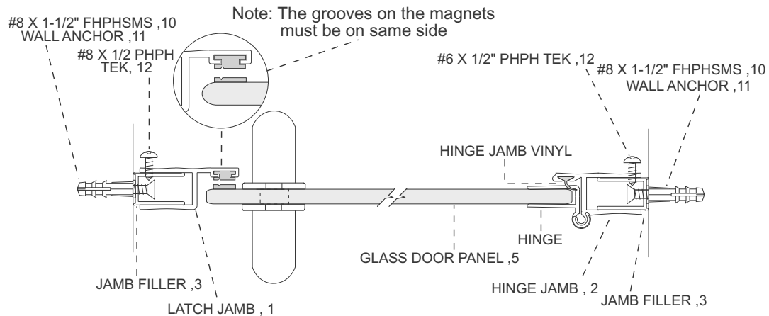
FIG. #3 - Shower Door Assembly - Top View
