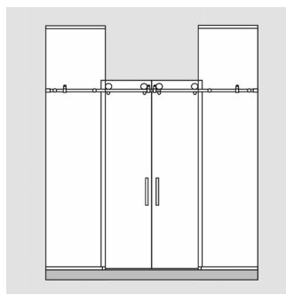
TRSE2280 Two door slider with two 180° panels to the ceiling
