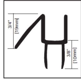
1/2" Std Door Sweep w/ Drip VN.4072.CLR - P912WS
