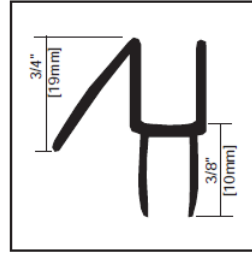
3/8" Std Door Sweep w/ Drip VN.4046.CLR - P990WS
