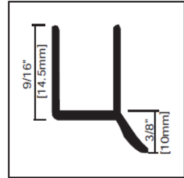
1/2" Seal Wipe VN.4074.CLR - P120WS
