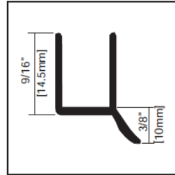
3/8" Seal Wipe VN.4037.CLR - P880WS
