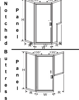
Handle / Full Height Magnetic Latch (2,6,7,8)
